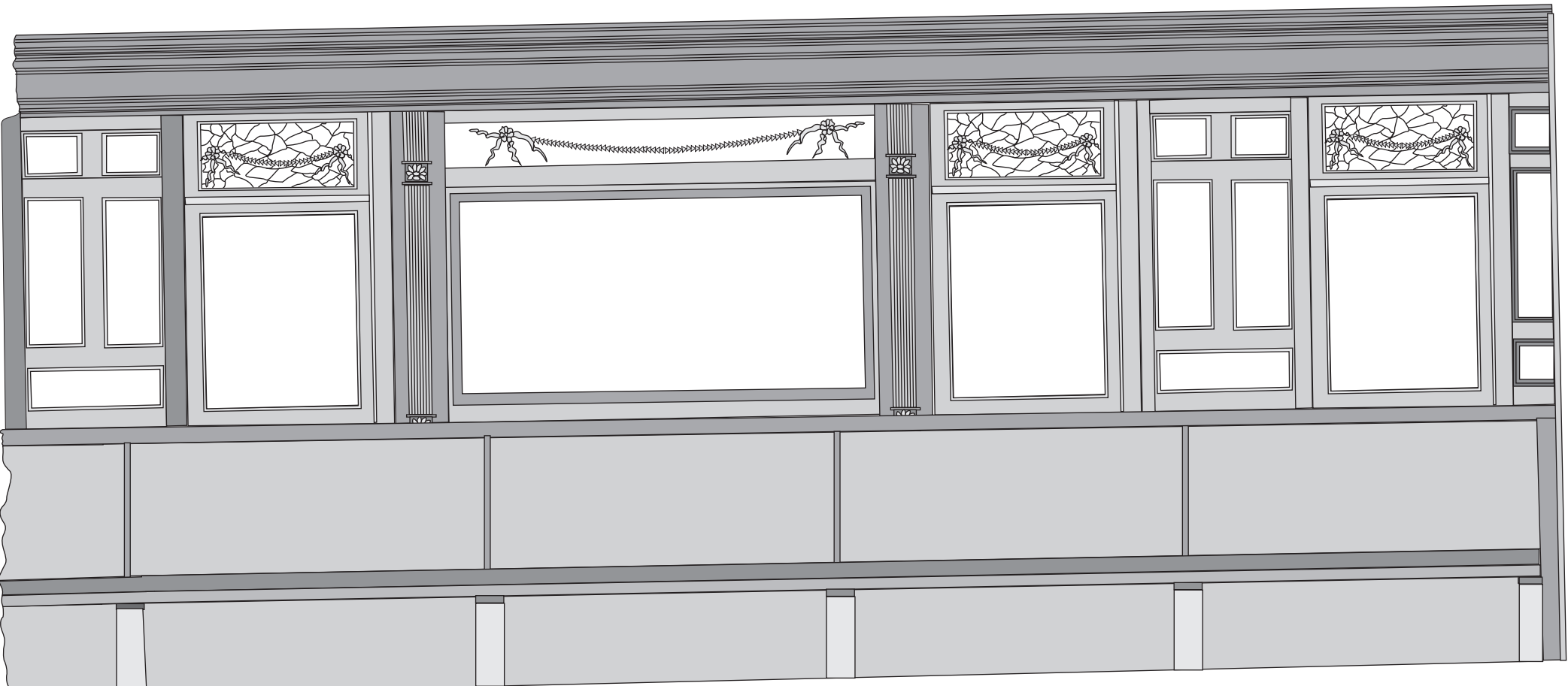
Looking inboard Ladies Cabin 1/2" Scale drawings for interior finish Ladies Cabin
