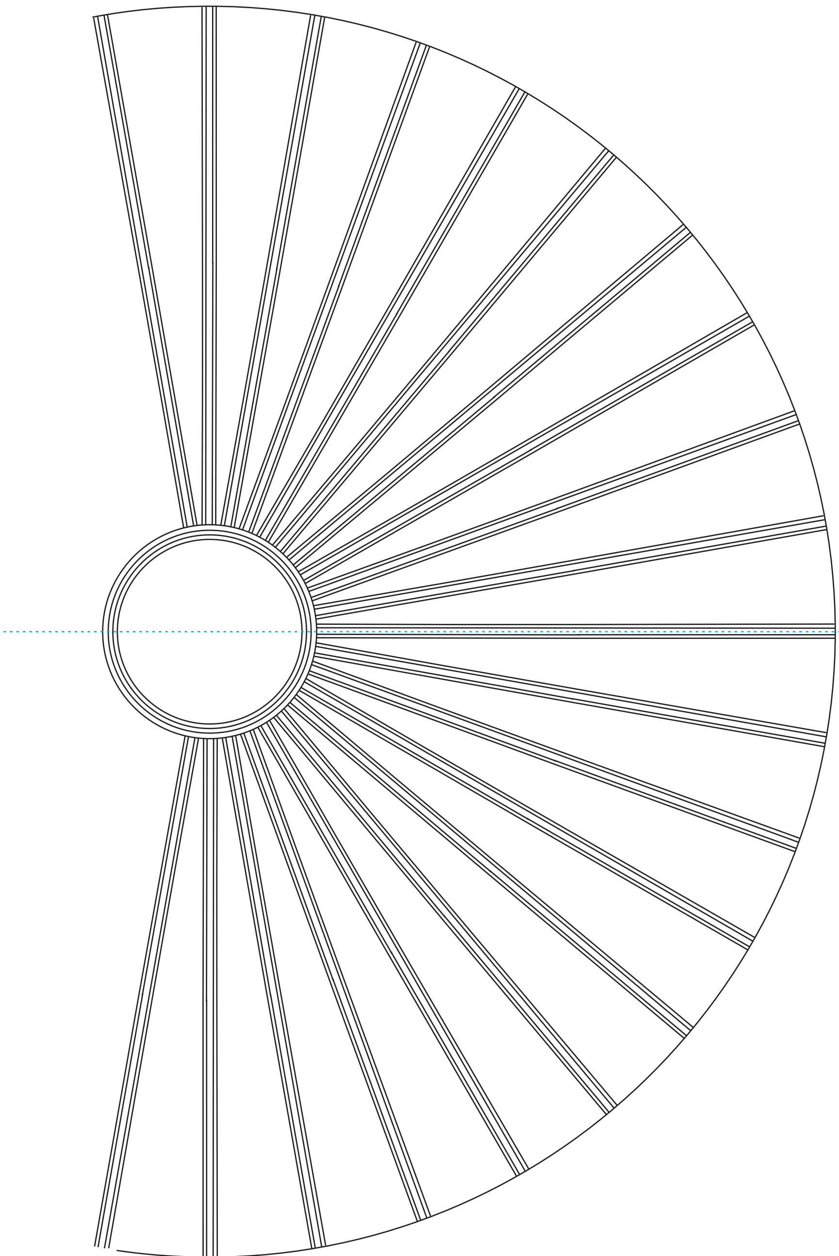
1/2" Scale Drawing Showing Radiating Carlings In Trunk Skylight
