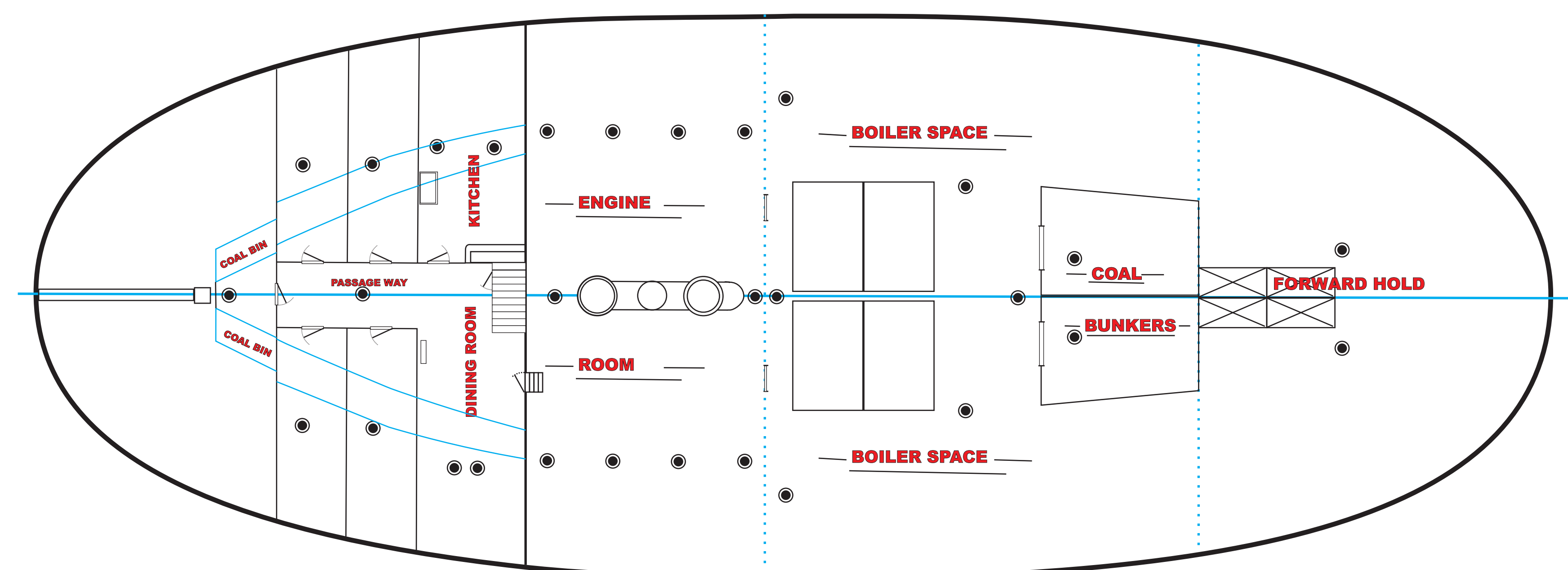
HOLD PLAN
